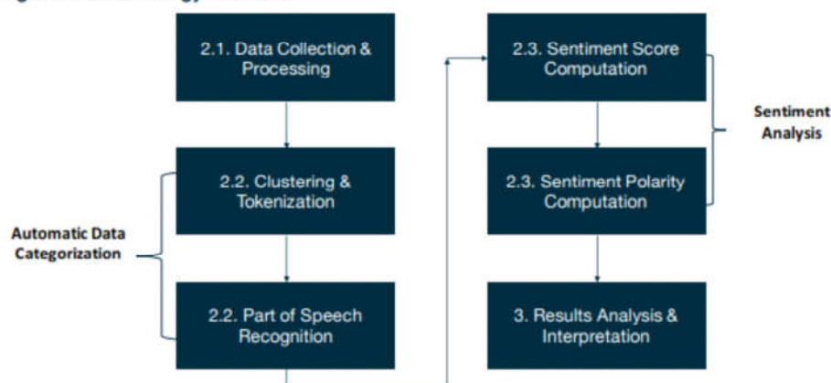
Figure 1: Methodology Overview
